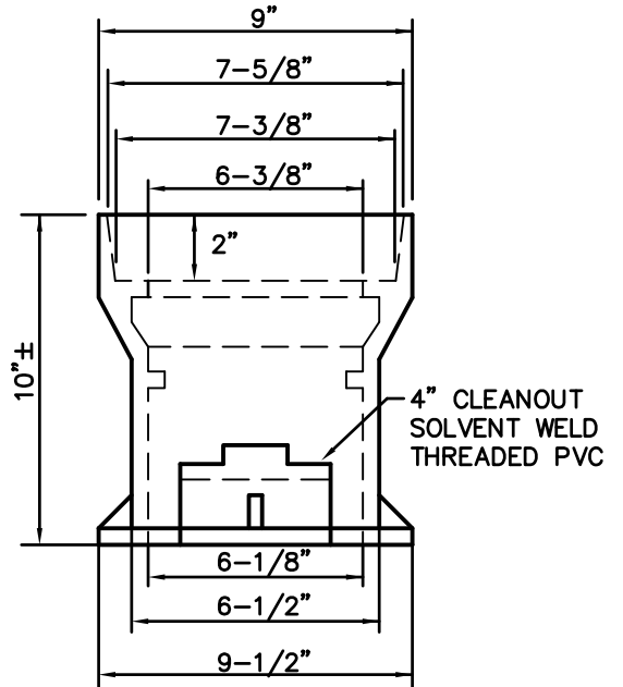
COVER DETAIL
